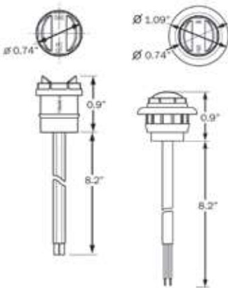
HOLE CUT-OUT: 0.75"
