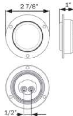
HOLE CUT-OUT: 2.313"
