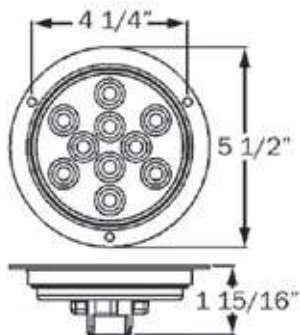
HOLE CUT-OUT: 4.5"
