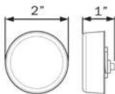
HOLE CUT-OUT: 2.313"
