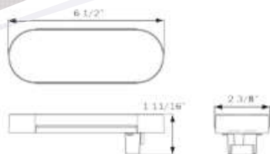
HOLE CUT-OUT: 6.85" x 2.5" (1.25" R)
