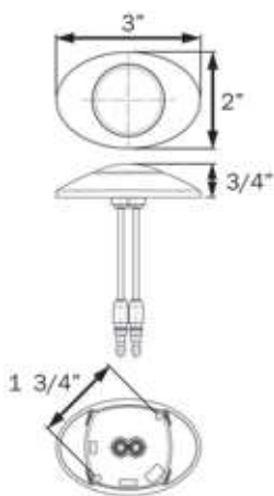
HOLE CUT-OUT: 1.375"
