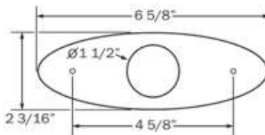
HOLE CUT-OUT: 1.5"
