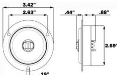
HOLE CUT-OUT: 2.75"
