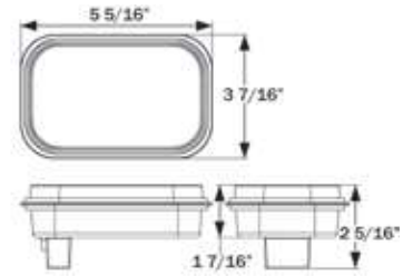
HOLE CUT-OUT: 5.462" x 3.562" (1" R)
