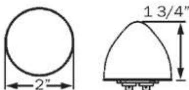
MCL21 SERIES HOLE CUT-OUT: 2.313"
