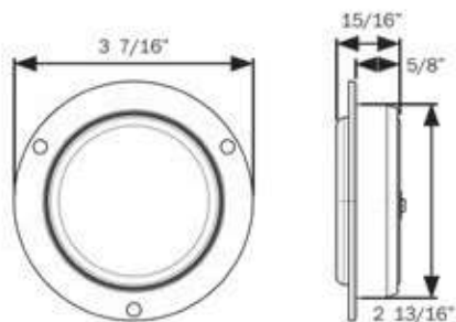
HOLE CUT-OUT: 2.75"
