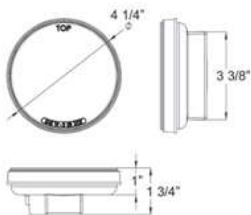
HOLE CUT-OUT: 4.5"
