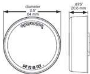
HOLE CUT-OUT: 2.75"
