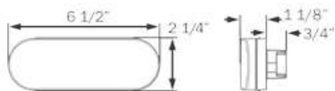
HOLE CUT-OUT: 6.85" x 2.5" (1.25" R)
