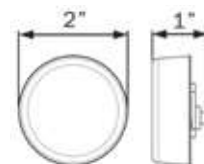
HOLE CUT-OUT: 2.313"
