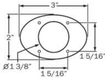
HOLE CUT-OUT: 1.375"
