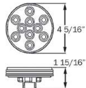
HOLE CUT-OUT: 4.5"
