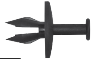
247-405 Std. Pkg. 20 pcs. Head Dia. 1", Stem Length: 23/32" GM 1982-on Fascia Retainer Fits into 3/8" Hole #14045480 CL Part No: 910-0565, Pieces: 3
