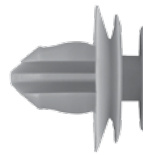
247-601 Std. Pkg. 25 pcs. Head Dia. 13mm, Stem Length: 11mm LEXUS 2000-on Garnish Moulding Retainer Stem Dia. 9mmx9mm, Overall Length: 18mm Middle Head Dia. 16mm, Bottom Head Dia. 18mm #90467-10167
