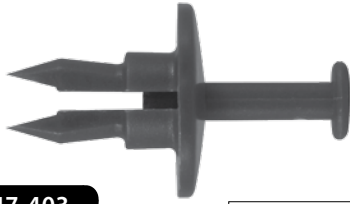
247-403 Std. Pkg. 25 pcs. Head Dia. 1", Stem Length: 7/8" GM 1982-on Fascia Retainer Shoulder Length: 1/4", Fits into 1/2" Hole #5973996 CL Part No: 910-0560, Pieces: 4
