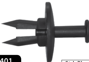
247-401 Std. Pkg. 15 pcs. Head Dia. 1", Stem Length: 3/4" GM 1979-on Fascia Retainer Shoulder Length: 1/8", Fits into 1/2" Hole #5973400 CL Part No: 910-0805, Pieces: 2
