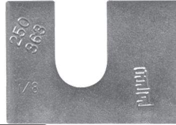
250-363 Std. Pkg. 25 pcs. 1-1/4"x1-3/4" Body Shim 1/2" Slot, 1/8" Thick CL Part No: 910-1725, Pieces: 4
